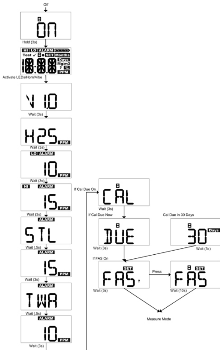
Fig. 4 Turning ON the instrument
