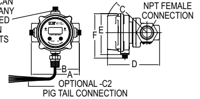
CTx (shown with -C2 pig tail connection)
