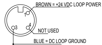
CX2 wire transmitter
