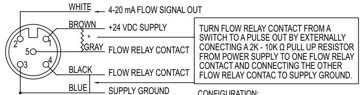
CX2 wire transmitter
