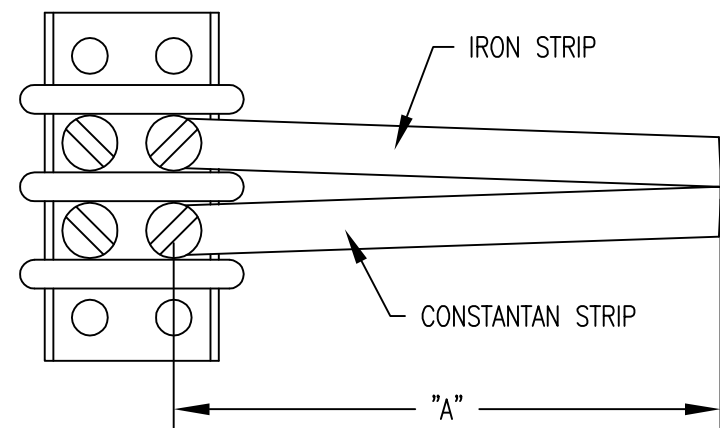
WEB TYPE WITH TERMINAL BLOCK
