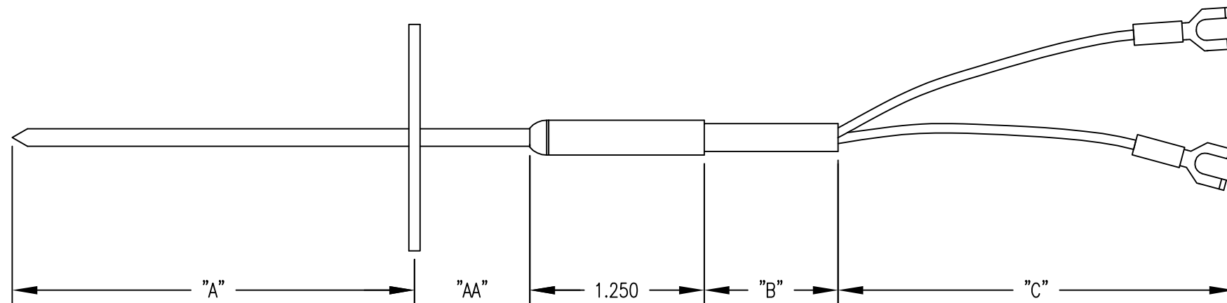
PENETRATION PROBE
