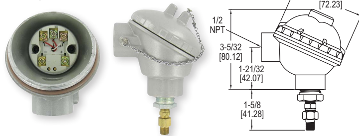
Accessory A-709 Transmitter Enclosure
