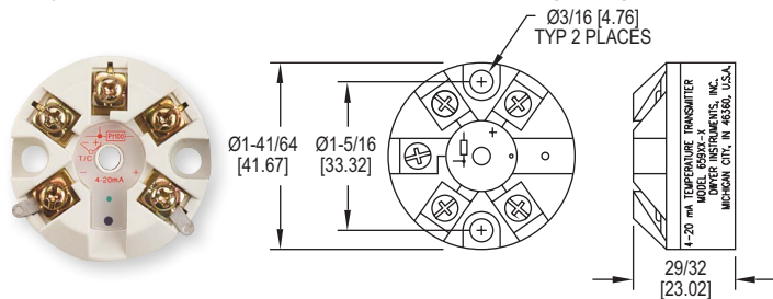
659 Transmitter
